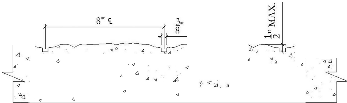
#901B 8x16 SPLIT BLOCK RAKED
